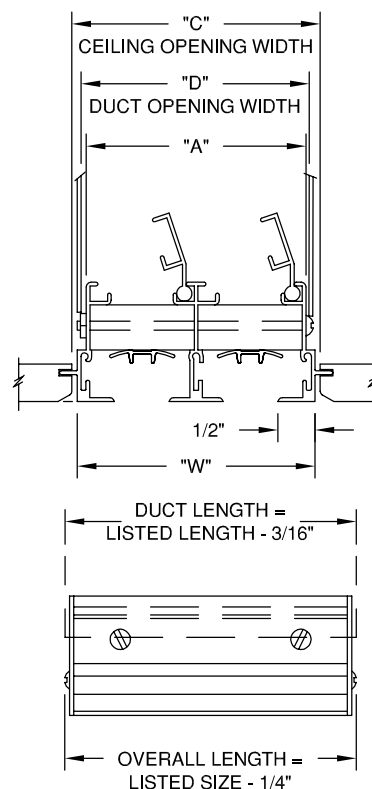
MODEL - 9475-670 CONCEALED SPLINE
